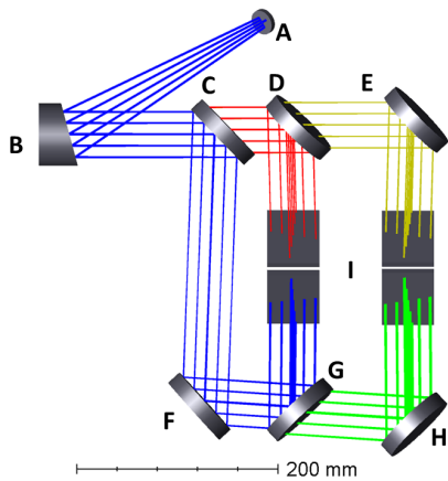
Figure 2. Left: Layout of the feed. A: Folding mirror; B: Off-axis parabola collimator; C/D/G: Dichroic mirrors dividing u + g from r + i , r from i , and u from g , respectively; E/F/H: Dielectric mirrors reflecting i , u + g , and g , respectively; I: gratings. Right: the as-built feed illuminated with a white light source.
